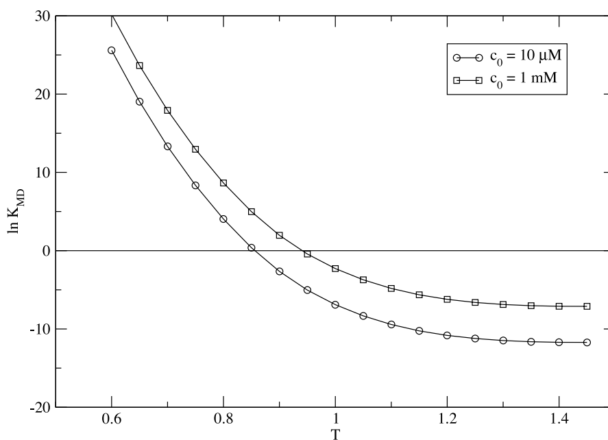
FIGURE 6 Equilibrium reaction constant for monomer-dimer equilibrium as a function of dimensionless temperature and for the two concentrations indicated.
