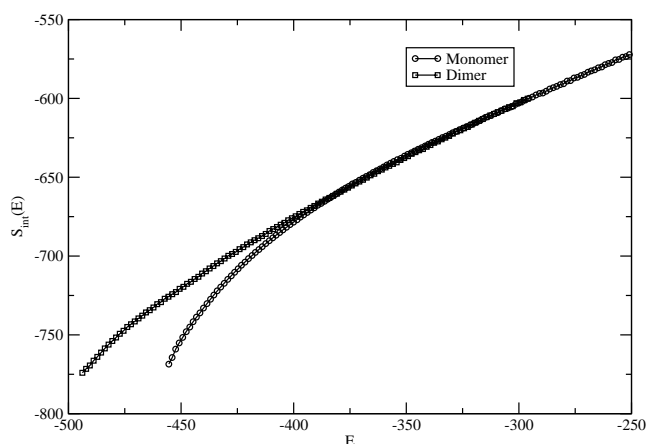
FIGURE 5 Rescaled internal entropy of the dimer S_{D,int} + S_0 , with S_0 = 52 (squares), and twice the internal entropy of the monomer 2S_{M,int}(E/2) (circles). The value of S_0 has been graphically determined to make the two curves coincide in the range of large E . As can be seen from the figure, the two curves superimpose quite accurately over a significant range of energies.
