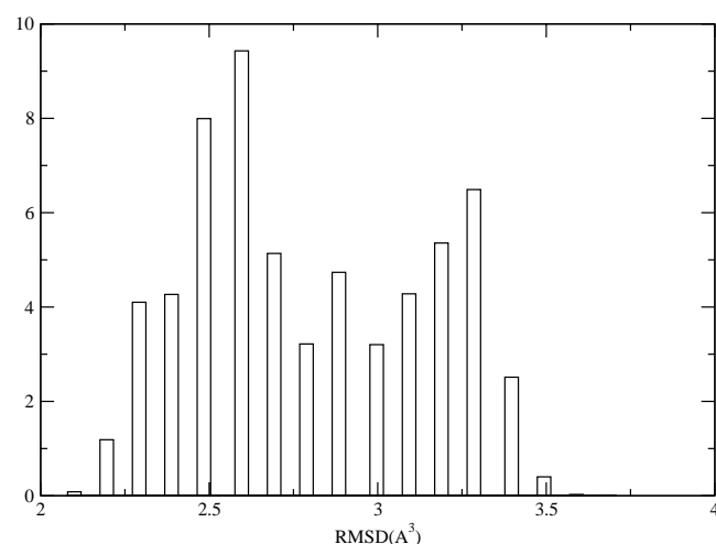
FIGURE 1 Histogram of the sampled root-mean-squared deviation from native (RMSD in \text{\AA}^3 at the dimensionless temperature T = 0.6 ).
