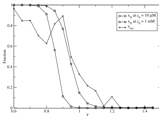
FIGURE 8 Equilibrium fraction of the dimer as a function of temperature. x_D = (1 + 4K_{\text{MD}} - \sqrt{1 + 8K_{\text{MD}}})/4K_{\text{MD}} , for the two concentrations indicated. The value of the equilibrium constant K_{\text{MD}} is shown in Fig. 6. We also show the fraction of configurations that, at the given temperature, had at least 50% native contacts.
